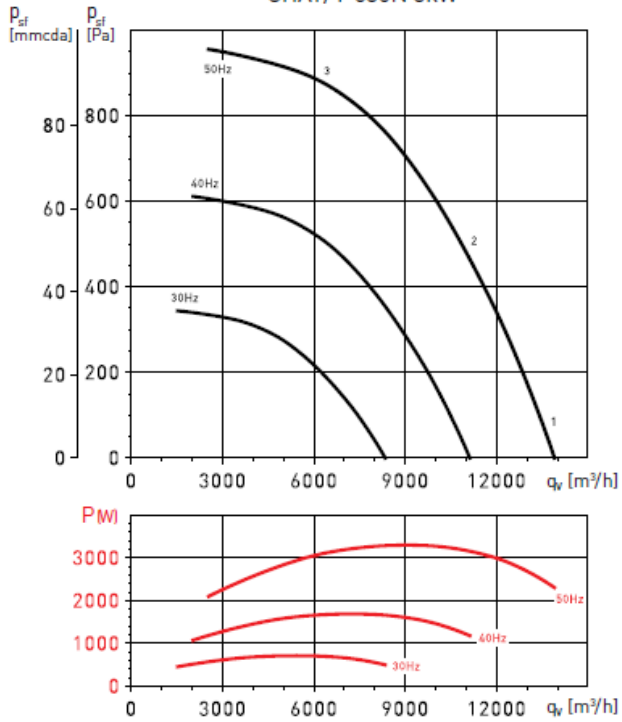
CHAT/4-630N 3kW
