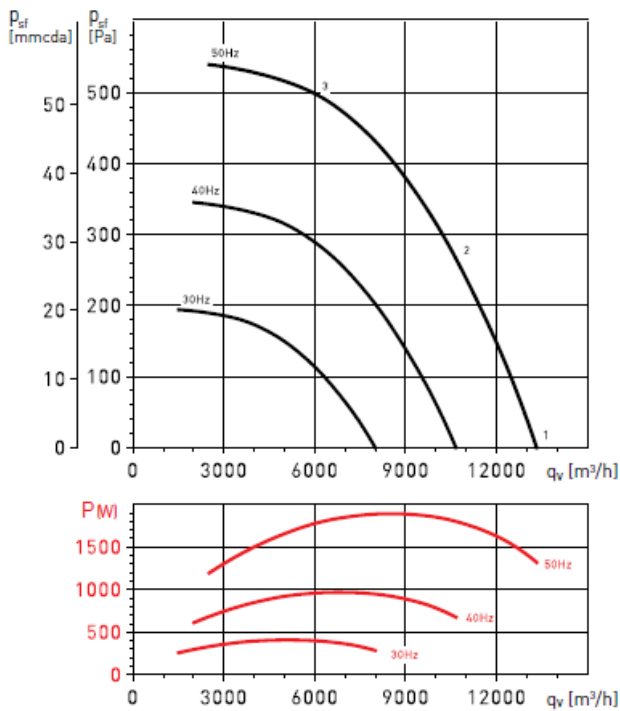
CHAT/6-710N 1,5kW
