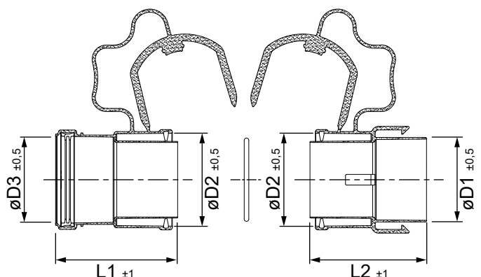
Manguito hembra Ø50/Ø60/Ø80/Ø100/Ø125
