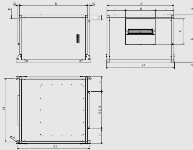
CVHT 9-10-12-15-18 Horizontal
