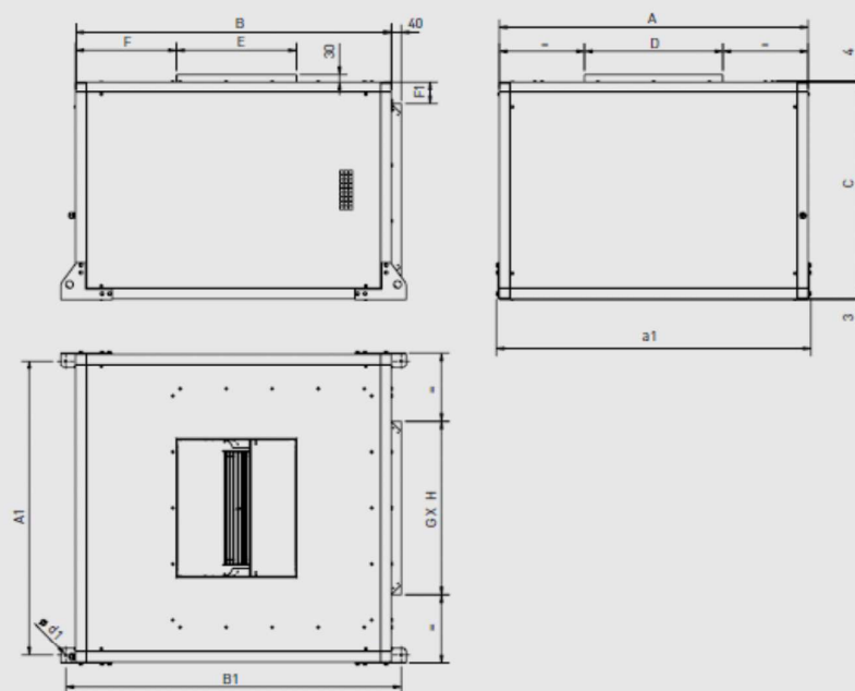
CVHT 9-10-12-15-18 Vertical
