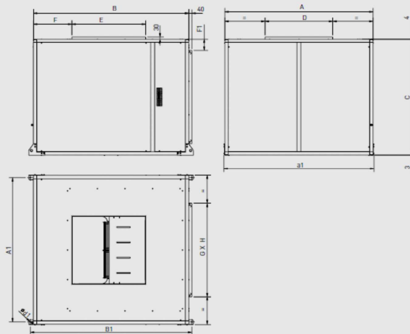
CVHT 20-22-25-30 Vertical
