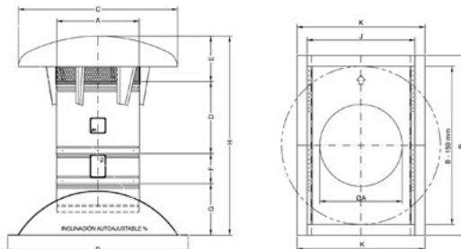
Security Fire - ABC-MU-TE-F400: 400°2H
